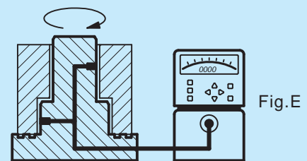
BORE to BORE RUNOUT (Using face as a secondary datum)
