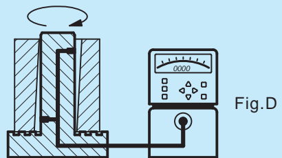
FACE to BORE RUNOUT
