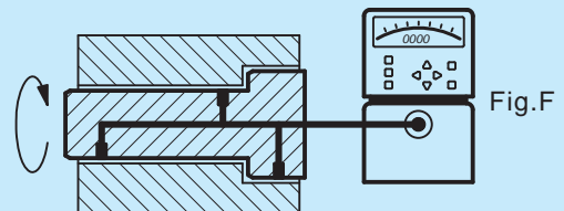
BORE to BORE RUNOUT (Using small bore for reference datum)
