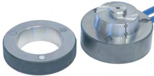
Dual circuit air taper probe mounted on base with setting master
